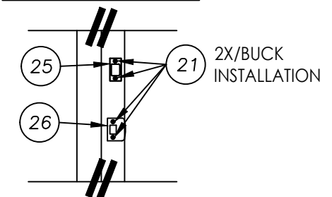
STRIKE DETAIL W/2X BUCK
