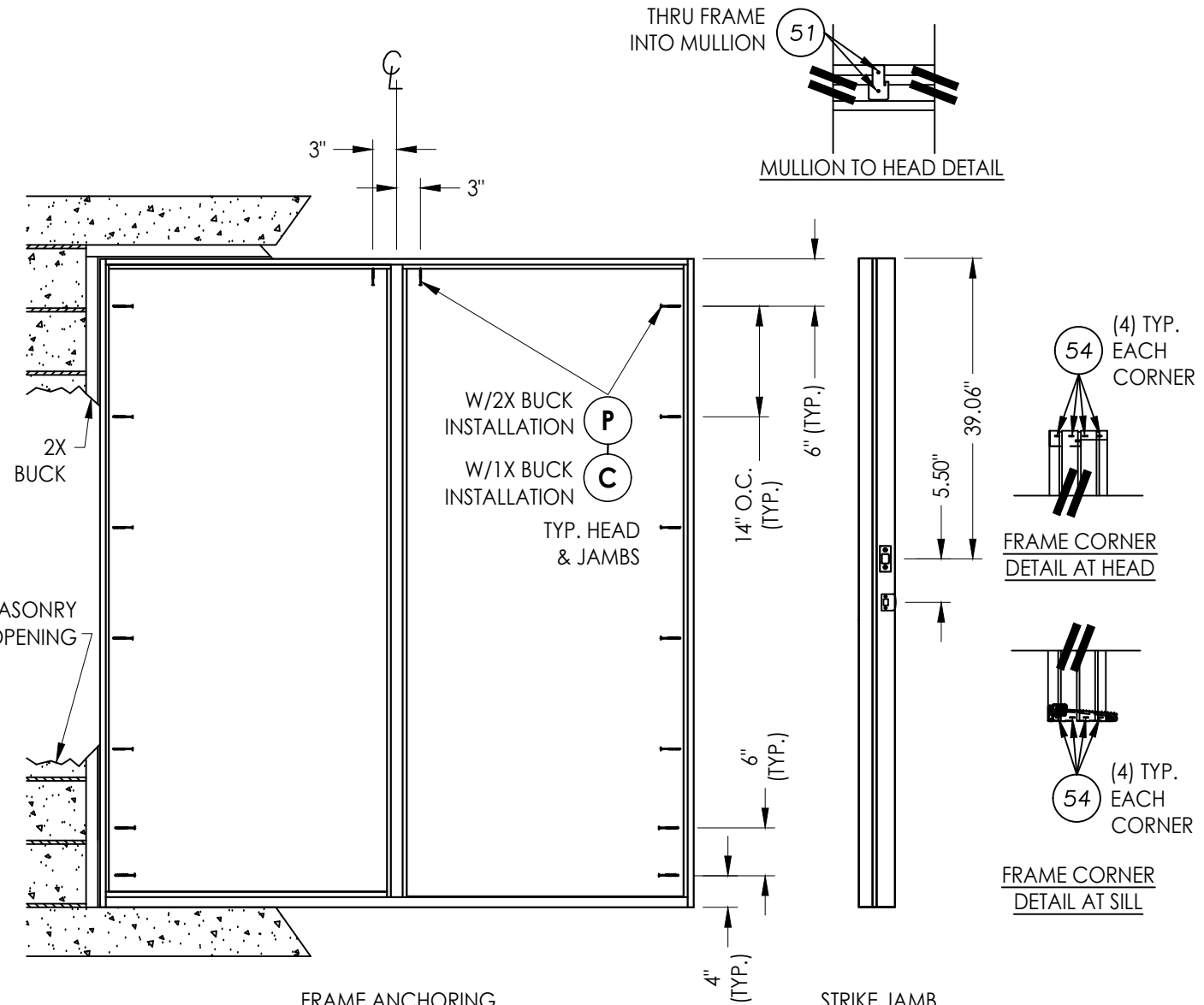
FRAME ANCHORING
