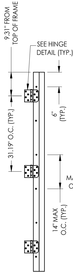
HINGE MULLION
