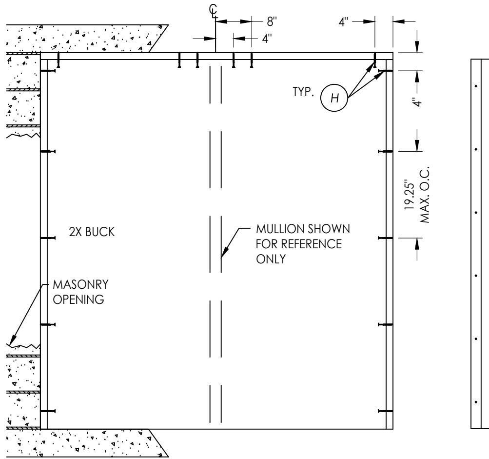
BUCK ANCHORING
